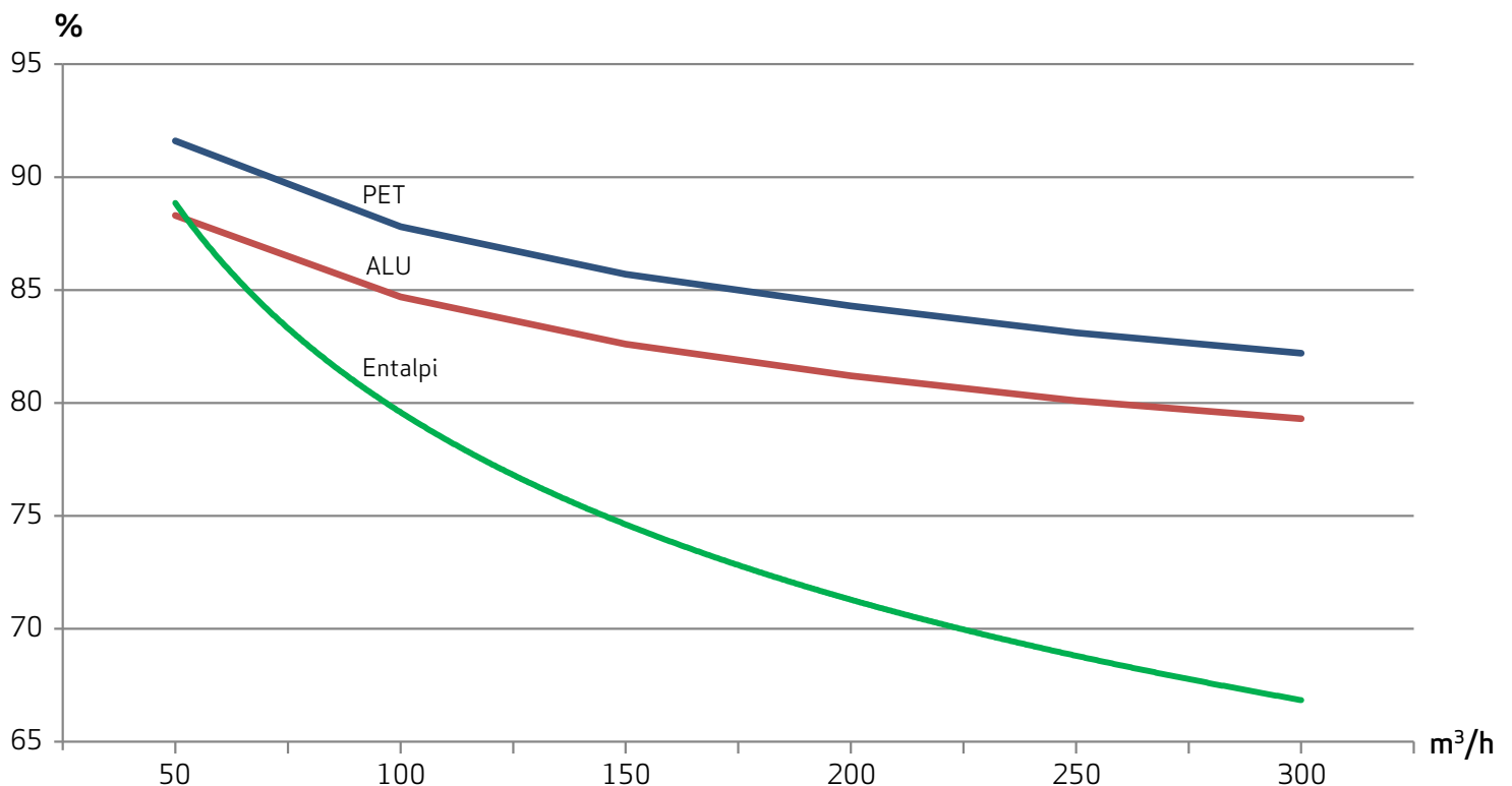
Temperature efficiency - measured according to EN308
